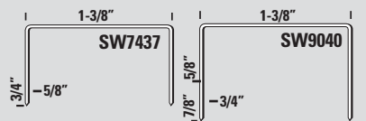
FASTENERS: 7237 SERIES, 9040 "A" CROWN STAPLES
