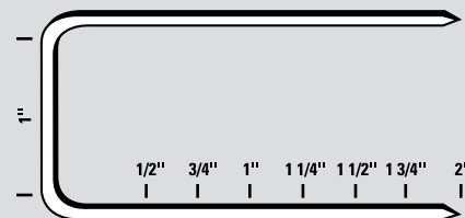
16-Gauge S2 Staple
